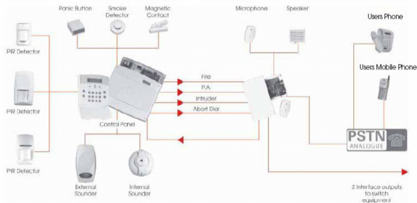
Bus Diagram
